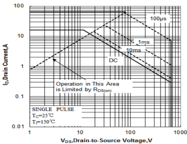
Fig 11 Safe Operating Area (TO-220AB / TO-263)
