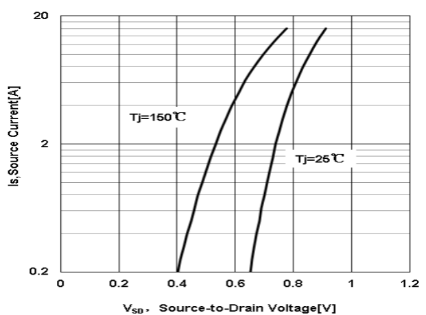
Fig 6 Body-Diode Characteristics
