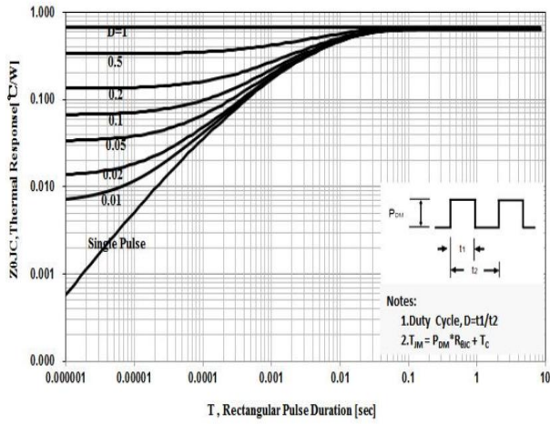
Fig 13 Maximum transient thermal impedance (TO-220AB / TO-263)
