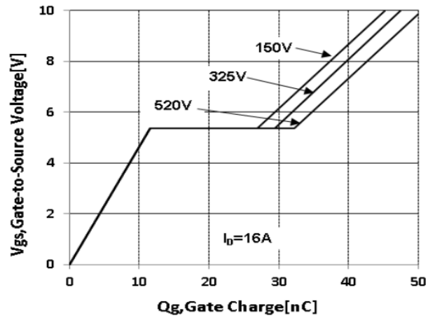
Fig 10 Gate-Charge Characteristics
