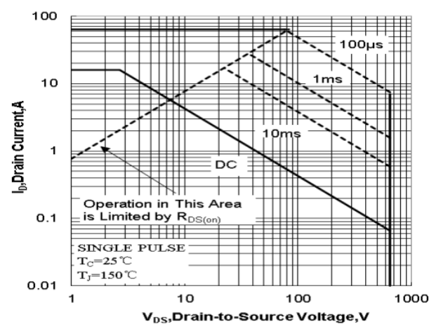
Fig 12 Safe Operating Area (ITO-220AB)
